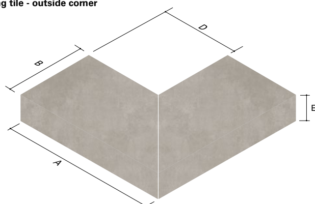
Schenkelplatte-Außenecke Nosing tile - outside corner
