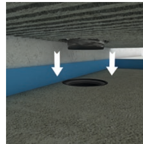
Apply wedi 320 tile adhesive to the underside of the wedi Fundo shower element and bond it to the floor.
